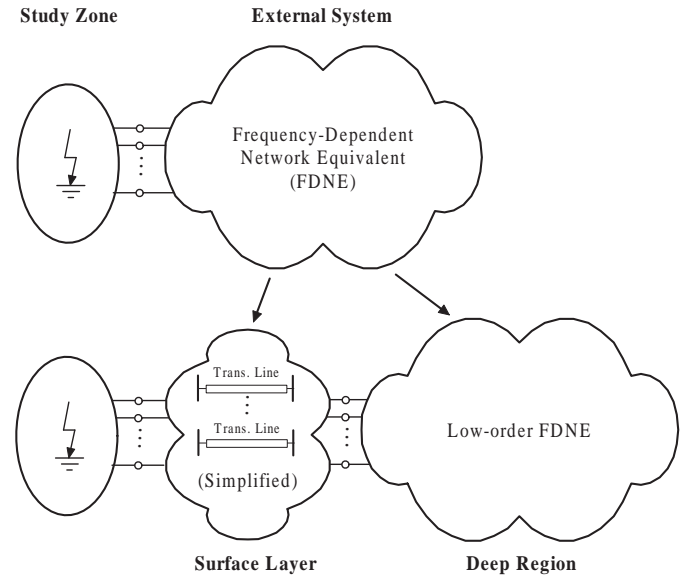
Fig. 1. Two-Layer Network Equivalent for an external system
