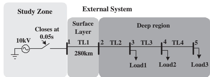
Fig. 14. Sample system diagram and partitioning for obtaining frequency response in Fig. 2
