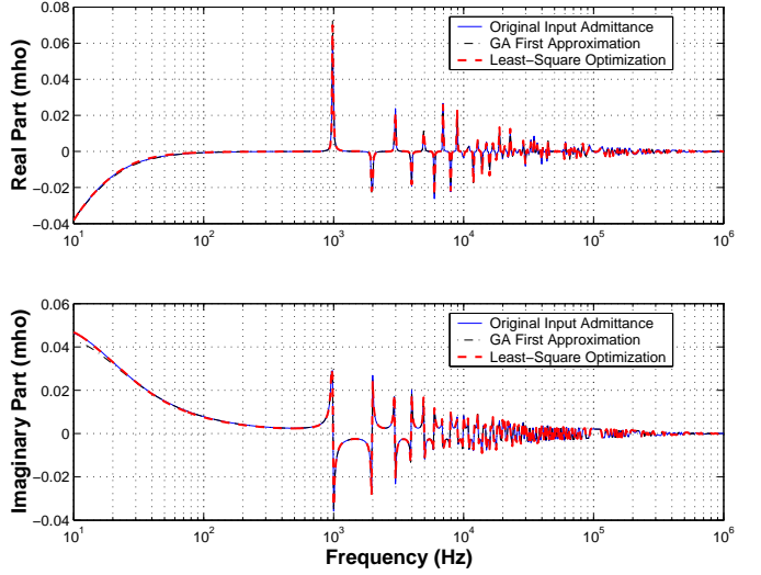
Fig. 10. Input admittance \mathbf{Y}_{input,12} in the Case Study
