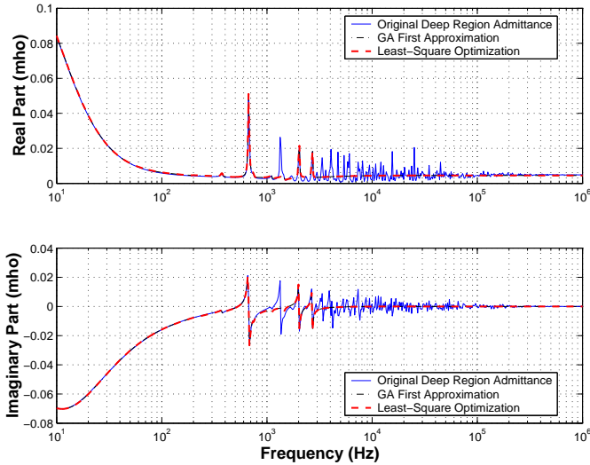
Fig. 8. Deep region admittance \mathbf{Y}_{deep,22} in the Case Study
