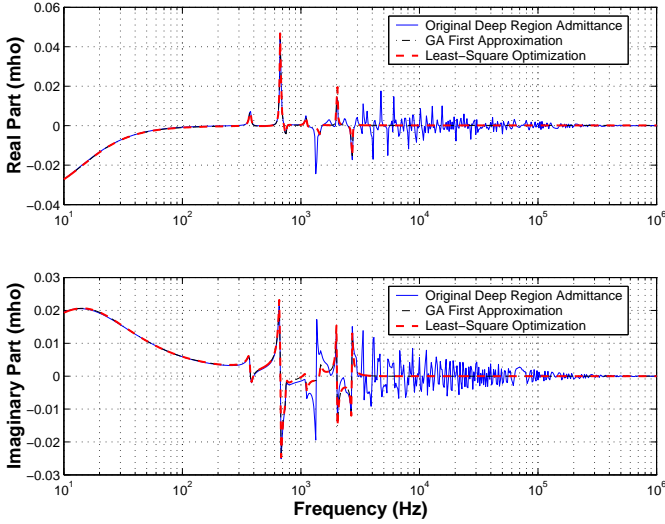
Fig. 7. Deep region admittance \mathbf{Y}_{deep,12} in the Case Study
