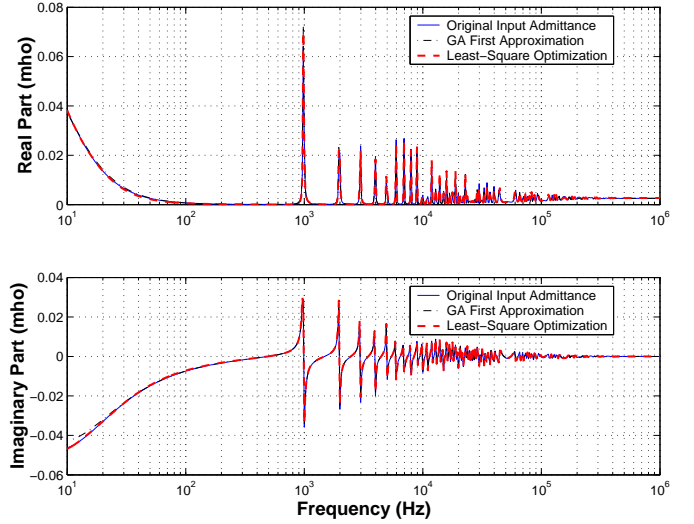
Fig. 9. Input admittance \mathbf{Y}_{input,11} in the Case Study
