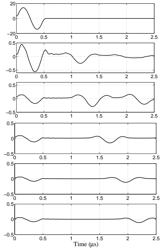
Fig. 8b. Computed inter-turn voltage distribution of turn 1-2 for transformer A
